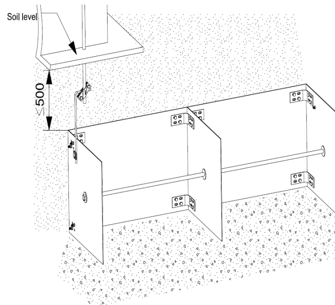
Installation of earth electrode type "E"™.
