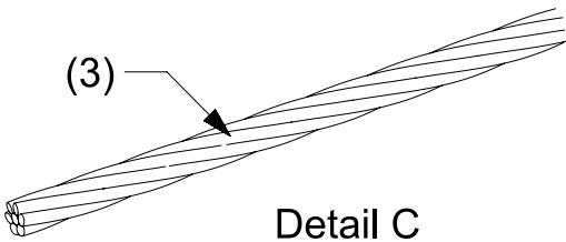
Detail C (3): Stranded copper conductor (Cu) 35mm², ELEMKO code 64 20 135 tested according IEC EN 62561 - 2
