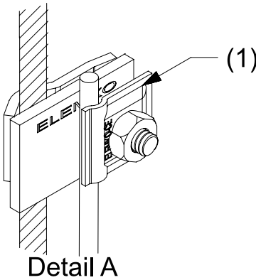
Detail A (1): St/tZn Clamp-fastener for earth termination system ELEMKO code 62 01 004 tested according IEC EN 62561 - 1
