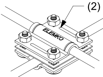
Detail B (2): Cu clamp with stainless steel screws , ELEMKO code 62 21 836 tested according IEC EN 62561 - 1, type H, 100kA, B1+B4,B2
